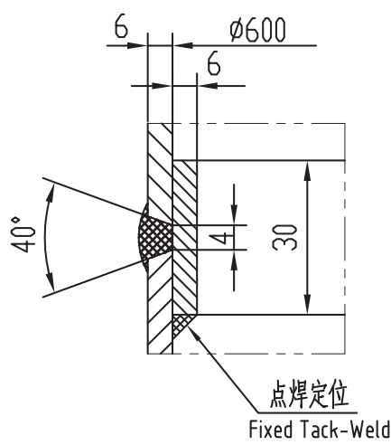
B1,B2 焊接详图 Welding detail of B1,B2 NO SCALE
