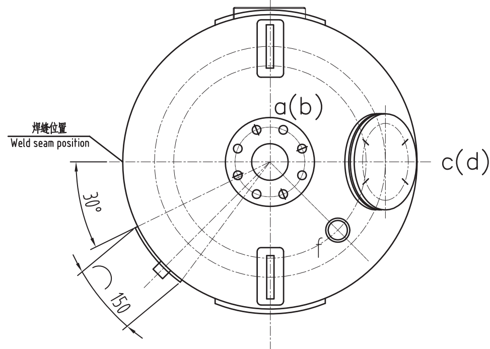
右吸附器方位图 Right adsorption cartridges diagram
