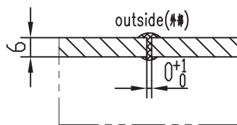
A1 焊接接详图 Welding detail of A1 NO SCALE
