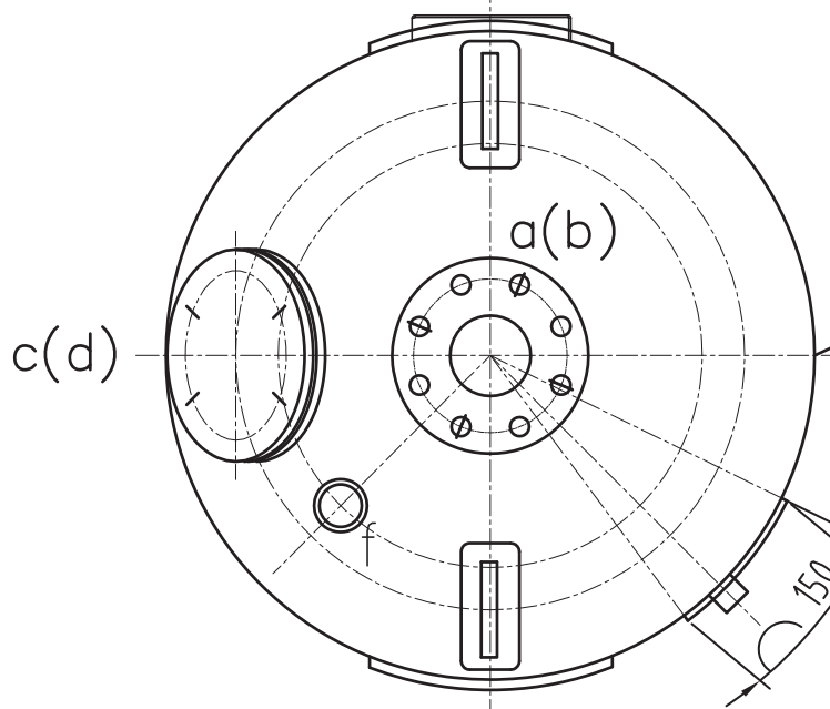
左吸附器方位图 Left adsorption cartridges diagram
