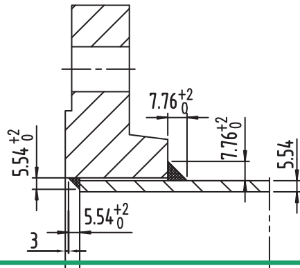
Welding detail of C3,C4 NO SCALE
